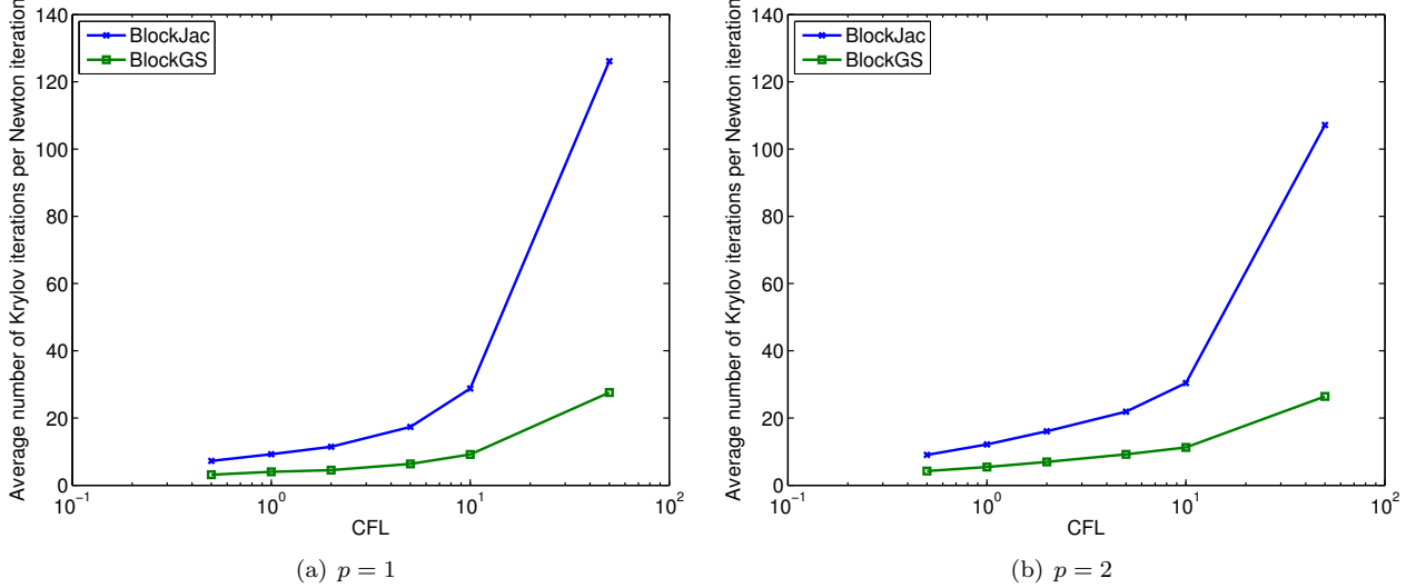
FIGURE 19. Number of Krylov iteration per Newton iteration for the vortex advection problem in dependence of the CFL number ( N_c = 3312 ).
