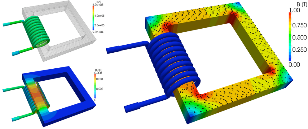
Fig. 19. Magnetostatic FEM-BEM coupling. Upper left: Given DC distribution j based on an excitation current I = 100\text{A} . Lower left: Excitation field B_0(j) as it is given in Eqn. (32). Right: The computed magnetic flux density B .
