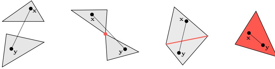
Fig. 6. Distinction of quadrature cases. From left to right: Regular integration: \tau_x and \tau_y feature a positive distance for all x and y . Vertex adjacent integration: \tau_x and \tau_y share a common point. Edge adjacent integration: \tau_x and \tau_y share a common edge. Coincident integration: \tau_x \equiv \tau_y .
