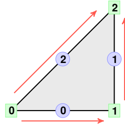
Fig. 4. Local numbering for BETL's RWG/Raviart-Thomas basis functions. Only lowest order edge functions for flat triangular elements are currently supported. The arrows indicate the edges' intrinsic positive orientations based on the element's node numbering ( from smaller to larger node index ).
