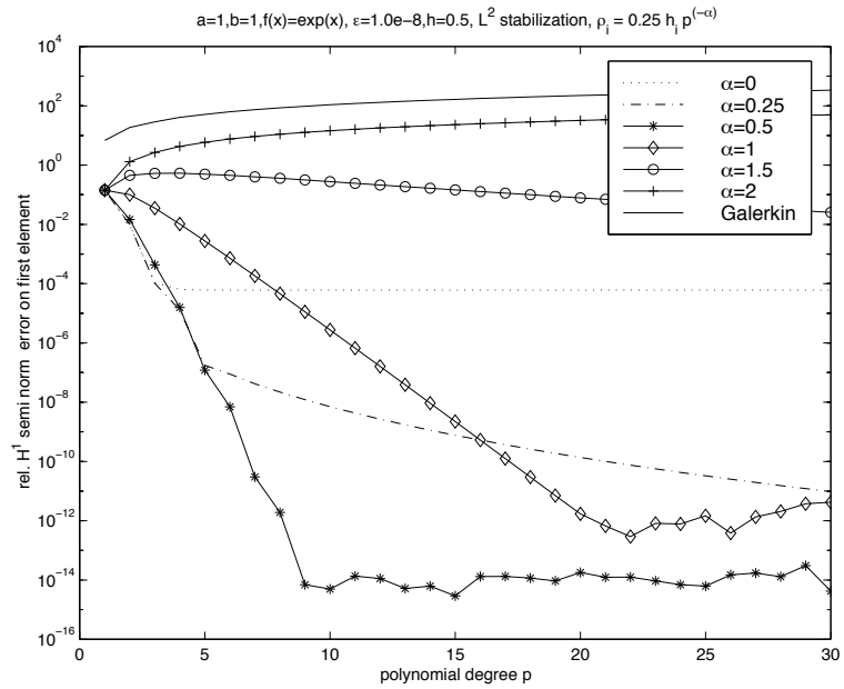
Figure 10: rel. error in H^1 semi norm performance on first element (-1, -1/2) for “ L^2 -stabilized” SDFEM for various choices of \rho_i ; \varepsilon = 10^{-8}
