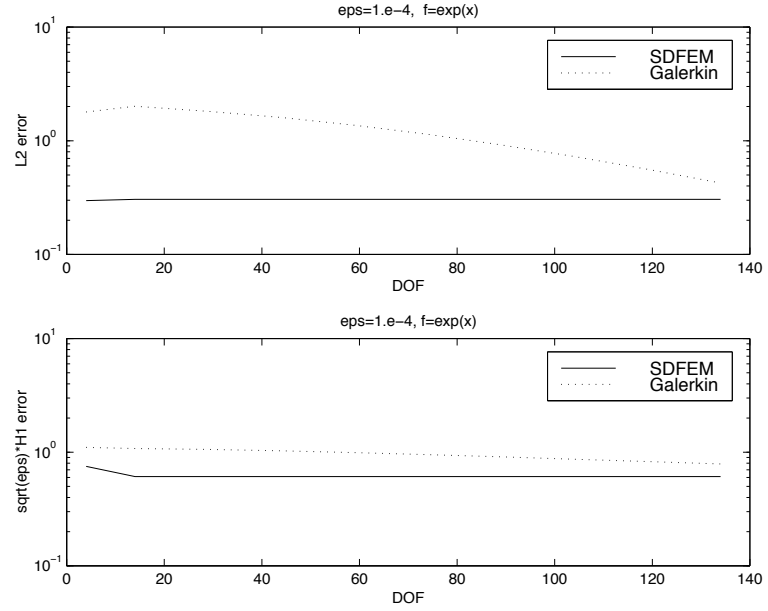
Figure 4: L^2 and energy performance of p version on uniform mesh with h = 0.5 + \text{small element size } \varepsilon , \varepsilon = 10^{-4}
