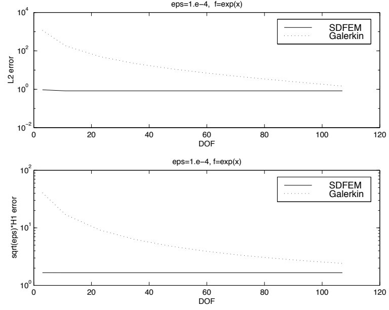
Figure 3: L^2 and energy performance of p version on uniform mesh with h = 0.5 for Galerkin FEM and “ L^2 -stabilized” SDFEM, \varepsilon = 10^{-4}
