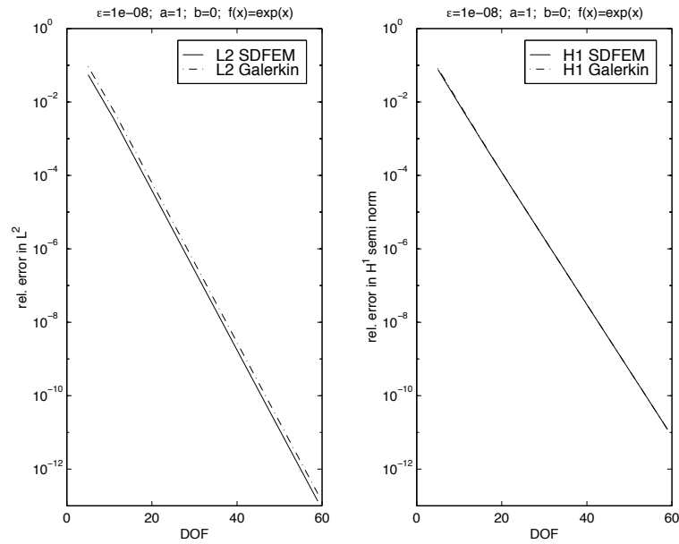
Figure 2: L^2 and energy performance of “two-element mesh” for Galerkin FEM and “ L^2 -stabilized” SDFEM, \epsilon = 10^{-8} ;
