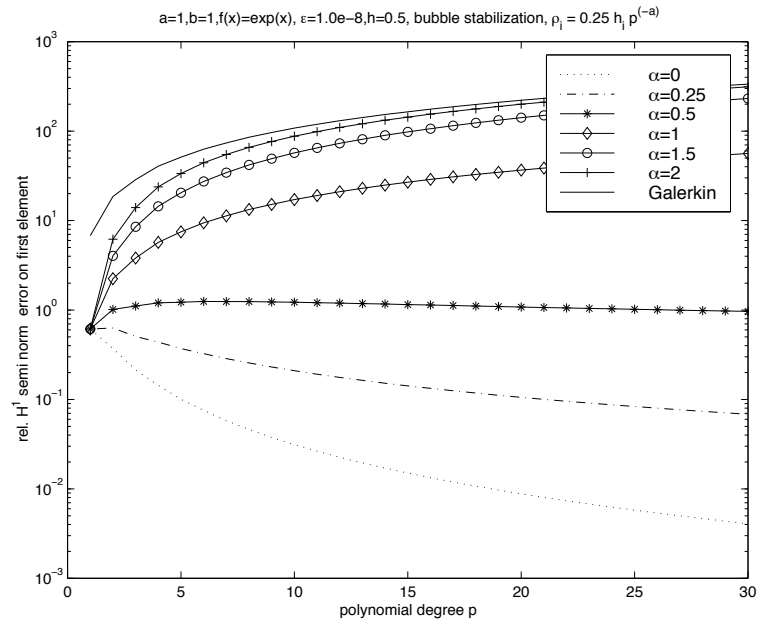
Figure 12: rel. error in H^1 semi norm performance on first element (-1, -1/2) for “bubble-stabilized” SDFEM for various choices of \rho_i ; \varepsilon = 10^{-8}
