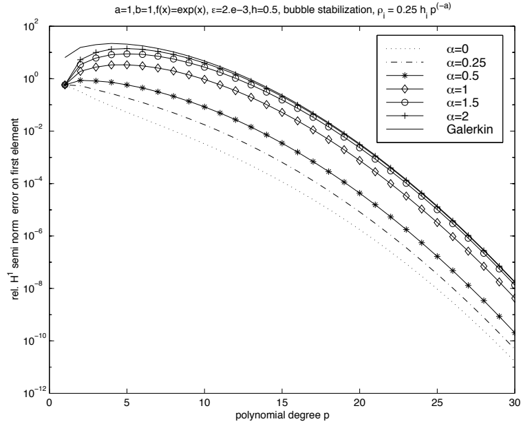
Figure 11: rel. error in H^1 semi norm performance on first element (-1, -1/2) for “bubble-stabilized” SDFEM for various choices of \rho_i ; \varepsilon = 2 \cdot 10^{-3}
